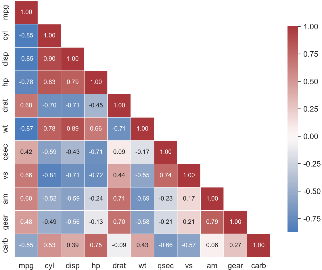
(B) Pearson Correlation Matrix of 11 Features
